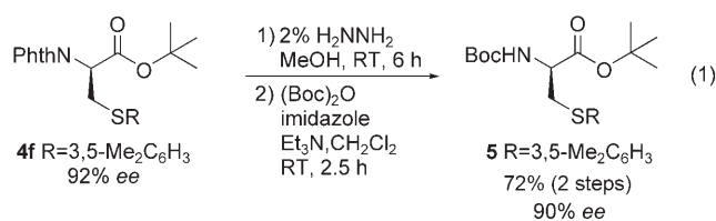
Scheme 3. Cleavage of the thioether.
